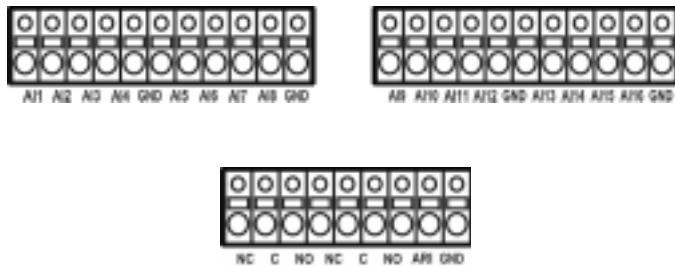
Figure G-1 I/O Connector Pinouts
