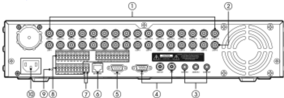
Figure 2-1 16-Channel DVR Rear Panel
