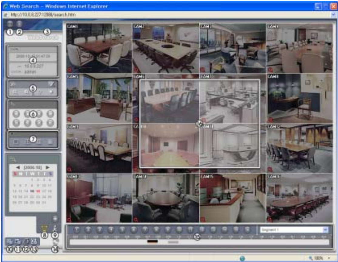
Figure D-3 WebSearch Screen
