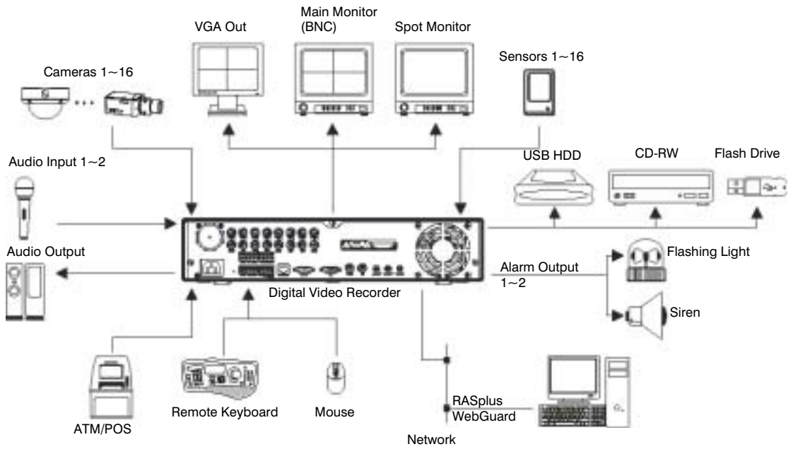
Figure 1-1 Typical DVR Installation for the HRSD8/16 DVR
