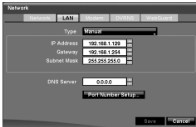
Figure 3-24 LAN (Manual) Setup Screen
